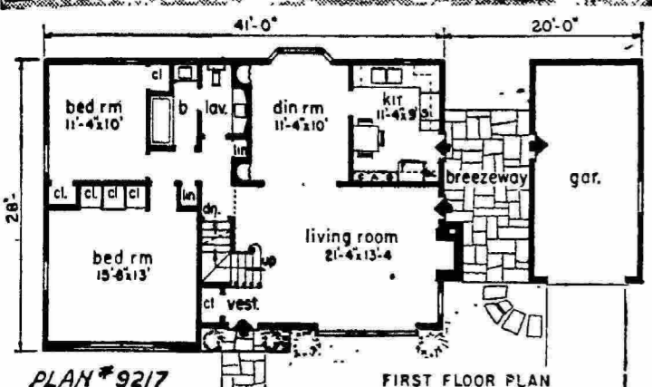
PLAN # 9217 FIRST FLOOR PLAN
